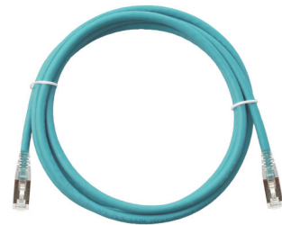
Ex. US-5201SLZ-9 : Shield CAT6A RJ45 to RJ45 Patch Cord, LSZH, Aqua blue, 1 meter
