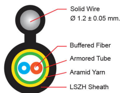
FTTH ROUND, ARMORED, STRANDED DROP CABLE
